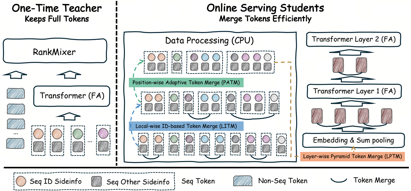
Figure 4: The overall framework of TM20K. Our model utilizes full attention (FA) for sequence modeling and RankMixer for heterogeneous token interaction. The teacher learns complete tokens without any token merge strategies, while the student models takes three simple yet well-motivated token merge strategies, including: (1) Local-wise ID-based Token Merge (LITM), (2) Position-wise Adaptive Token Merge (PATM), and (3) Layer-wise Pyramid Token Merge (LPTM).
