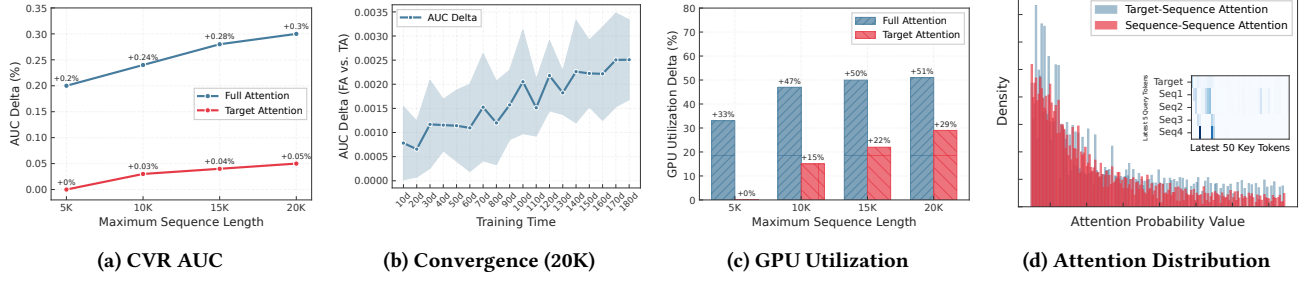
Figure 2: Comparisons between full attention (FA) and target attention (TA) from multiple aspects.
