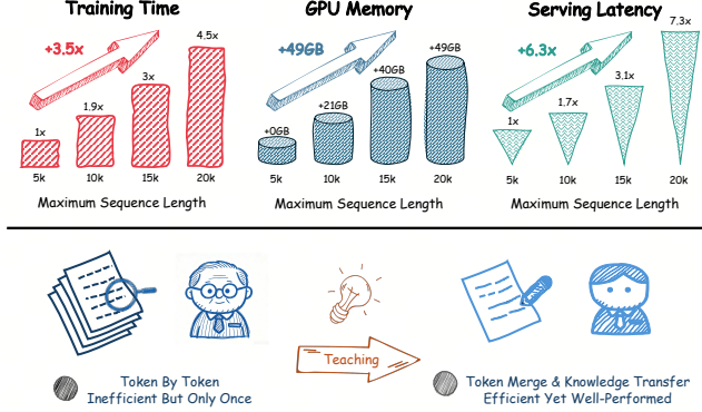
Figure 1: The motivation of TM20K. Ultra-long sequence modeling introduces significant burdens on training time, GPU memory, and serving latency. TM20K offloads heavy computation to a one-time trained teacher model that preserves all original tokens, enabling the student models to train and serve efficiently via well-motivated token merge strategies and the knowledge transferred from the teacher.
