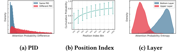
Figure 3: Statistics and visualization of attention scores calculated from a subset of training instances.
